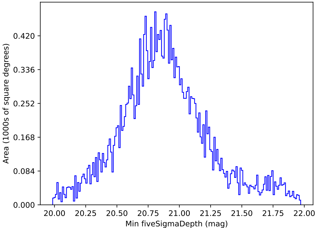
roll_pause_mjdp180_v3.4_10yrs All sky all bands: Min fiveSigmaDepth
