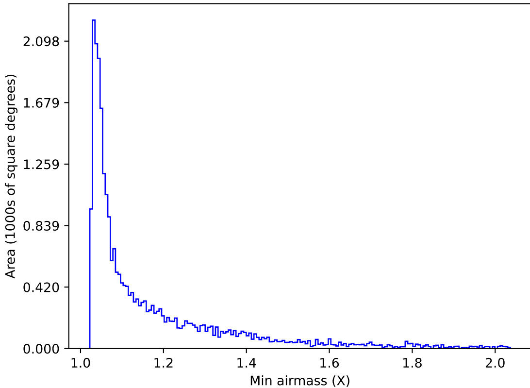
roll_pause_mjdp180_v3.4_10yrs Yr 1 z band: Min airmass
