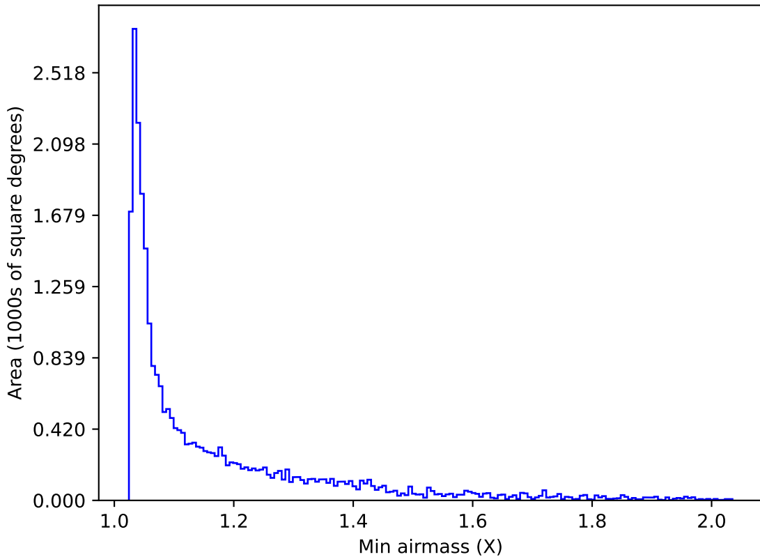
roll_pause_mjdp180_v3.4_10yrs Yr 1 r band: Min airmass
