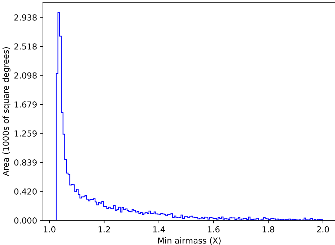
roll_pause_mjdp180_v3.4_10yrs Yr 1 i band: Min airmass
