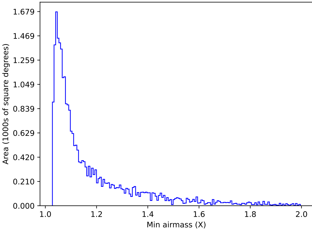
roll_pause_mjdp180_v3.4_10yrs Yr 1 g band: Min airmass
