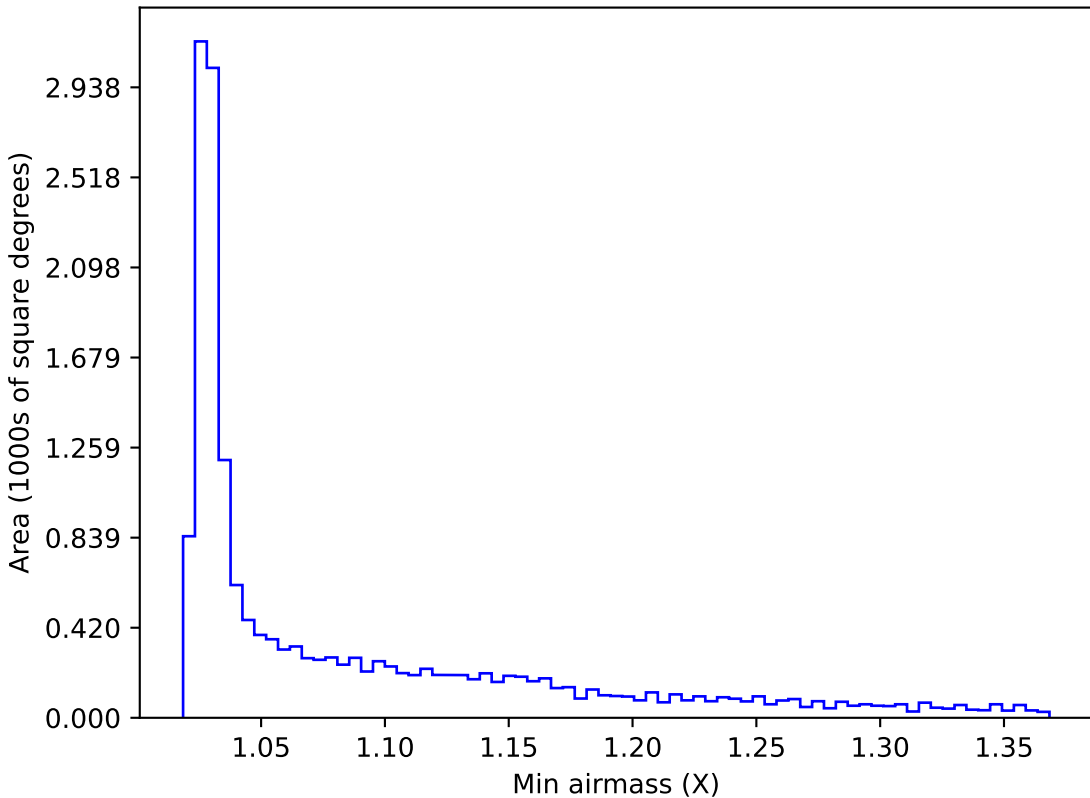
roll_pause_mjdp180_v3.4_10yrs WFD z band: Min airmass
