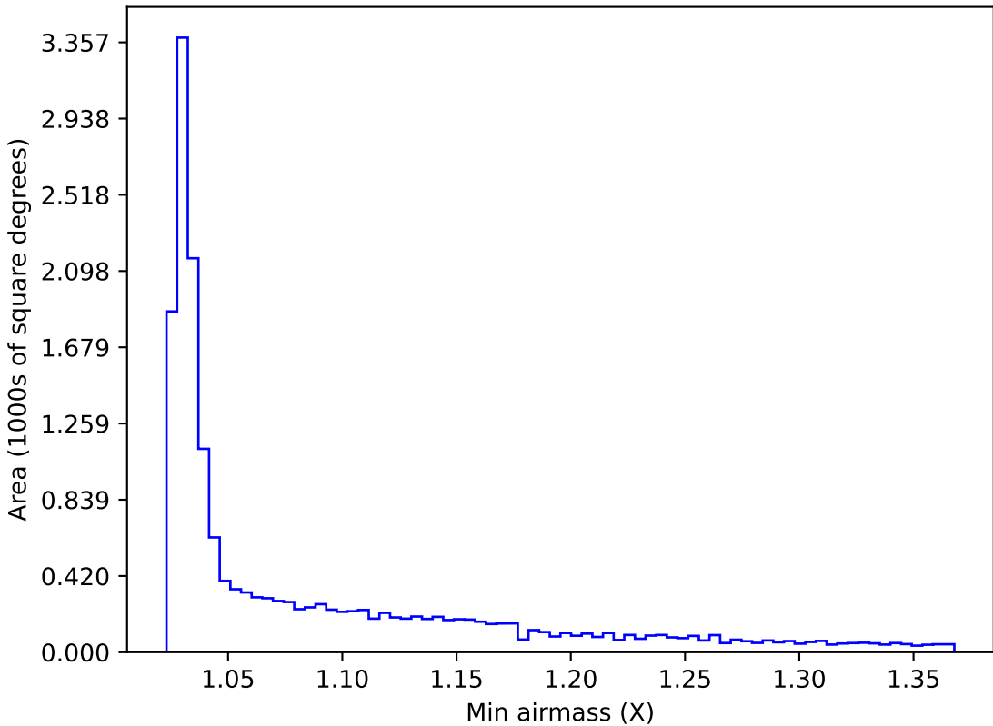
roll_pause_mjdp180_v3.4_10yrs WFD y band: Min airmass
