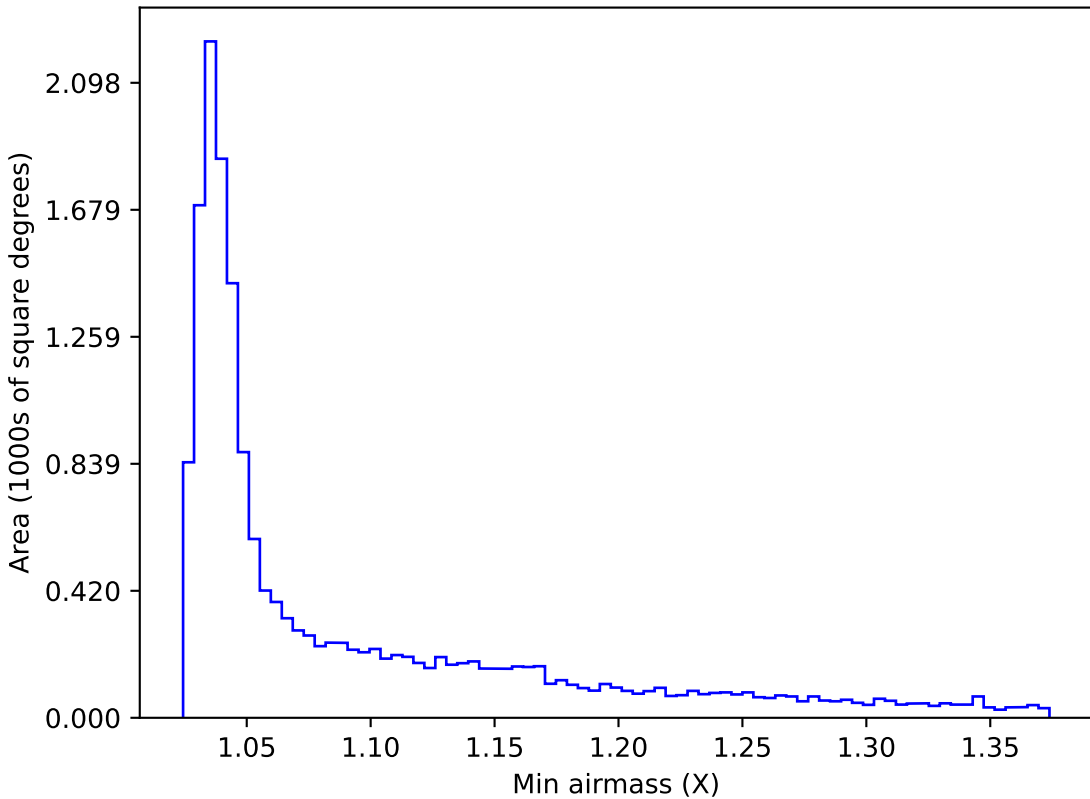
roll_pause_mjdp180_v3.4_10yrs WFD u band: Min airmass
