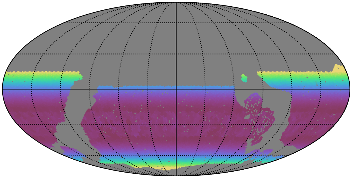
roll_pause_mjdp180_v3.4_10yrs WFD g band: Min airmass
