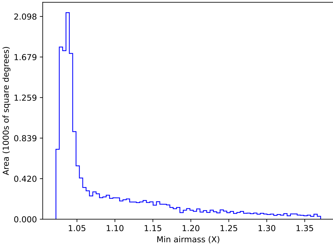
roll_pause_mjdp180_v3.4_10yrs WFD g band: Min airmass
