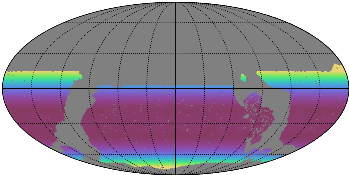
roll_pause_mjdp180_v3.4_10yrs WFD all bands: Min airmass
