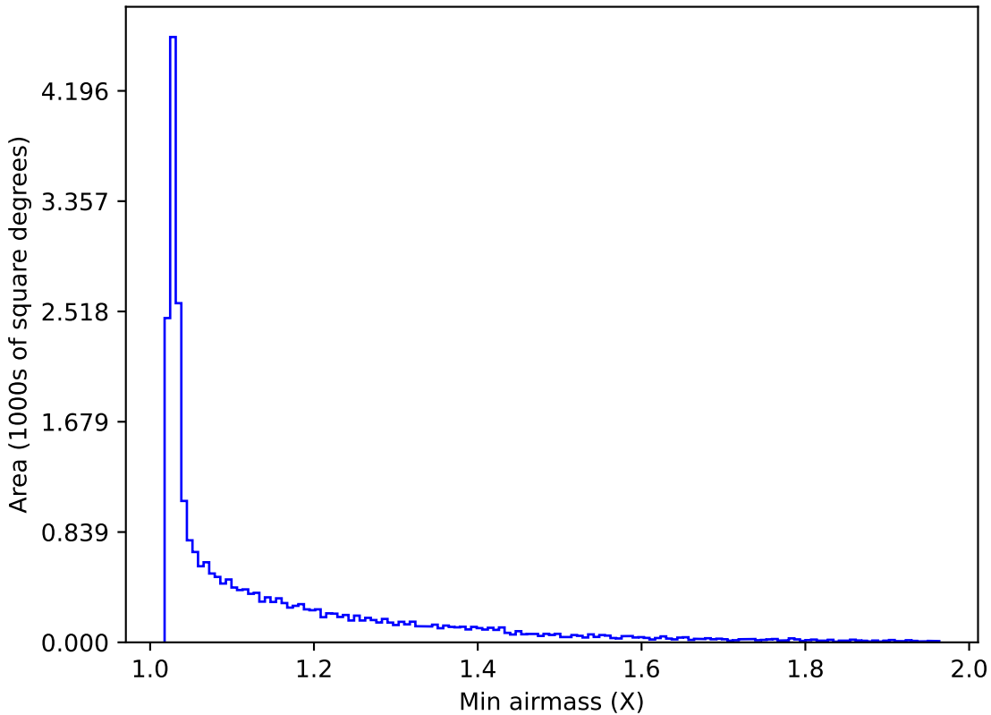
roll_pause_mjdp180_v3.4_10yrs All sky r band: Min airmass
