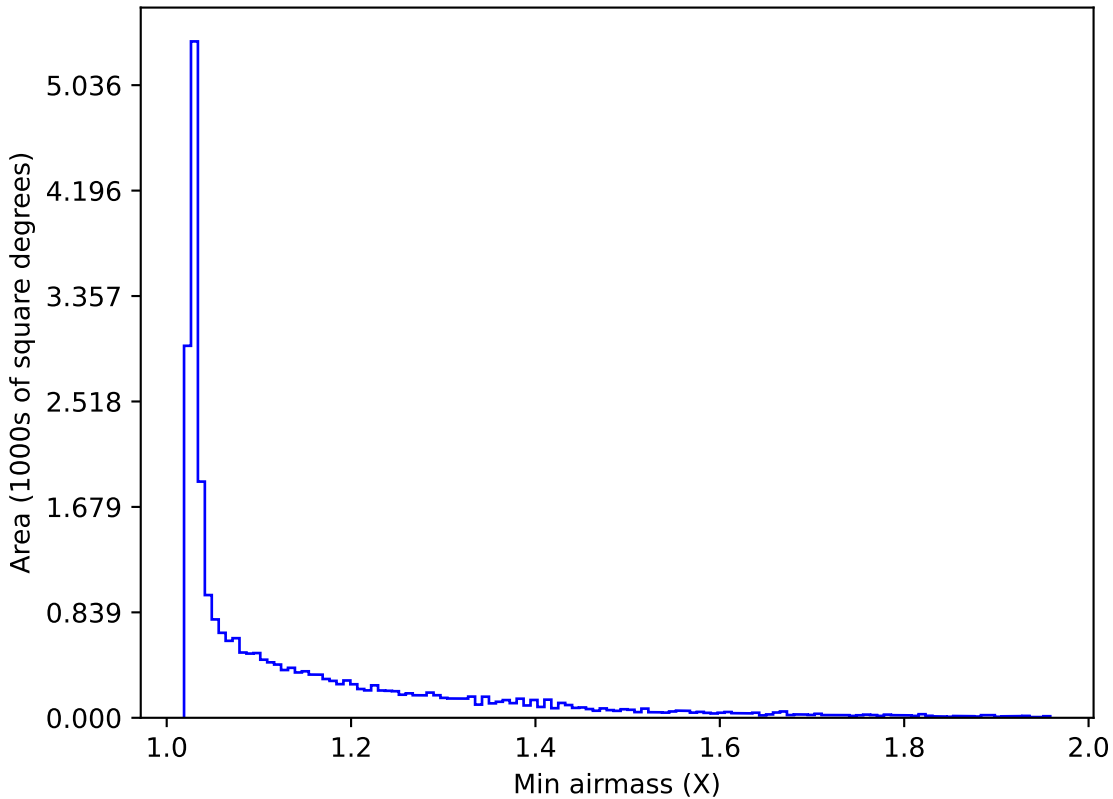
roll_pause_mjdp180_v3.4_10yrs All sky i band: Min airmass
