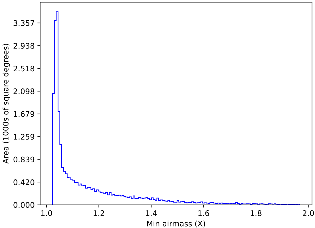
roll_pause_mjdp180_v3.4_10yrs All sky g band: Min airmass
