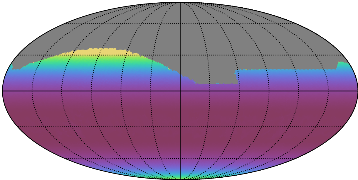
roll_pause_mjdp180_v3.4_10yrs All sky all bands: Min airmass
