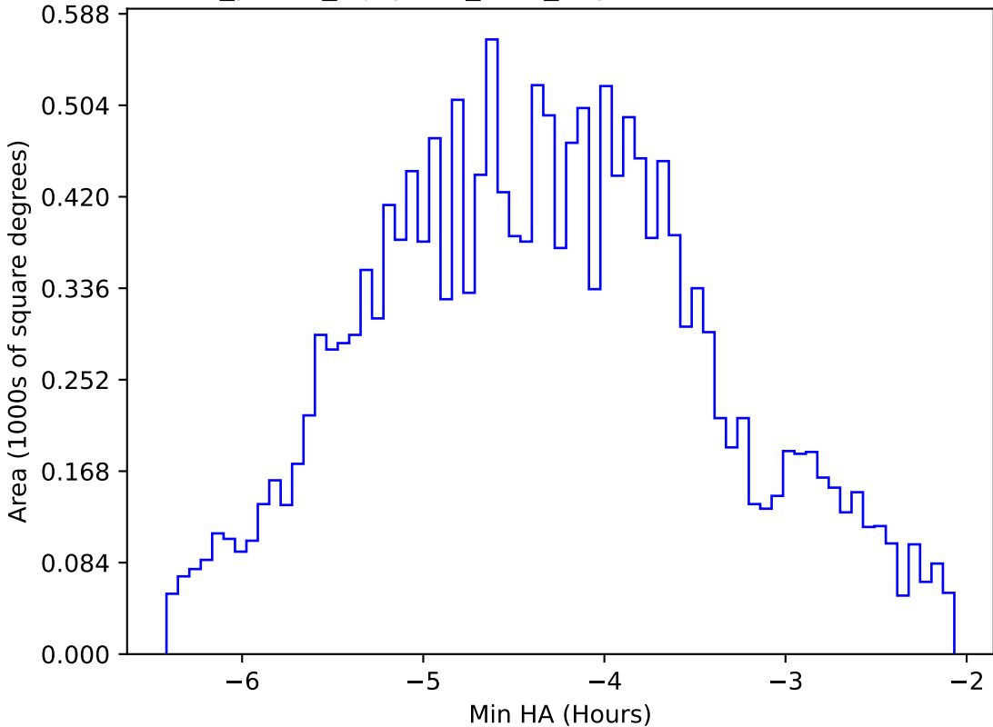
roll_pause_mjdp180_v3.4_10yrs WFD z band: Min HA
