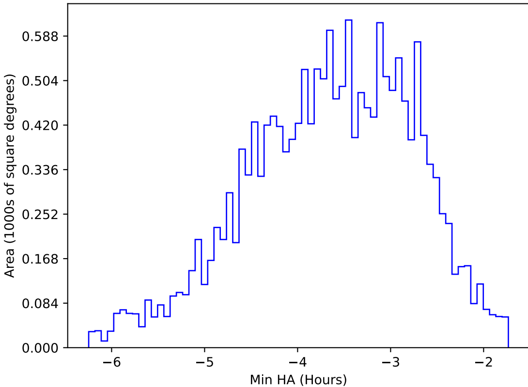
roll_pause_mjdp180_v3.4_10yrs WFD y band: Min HA
