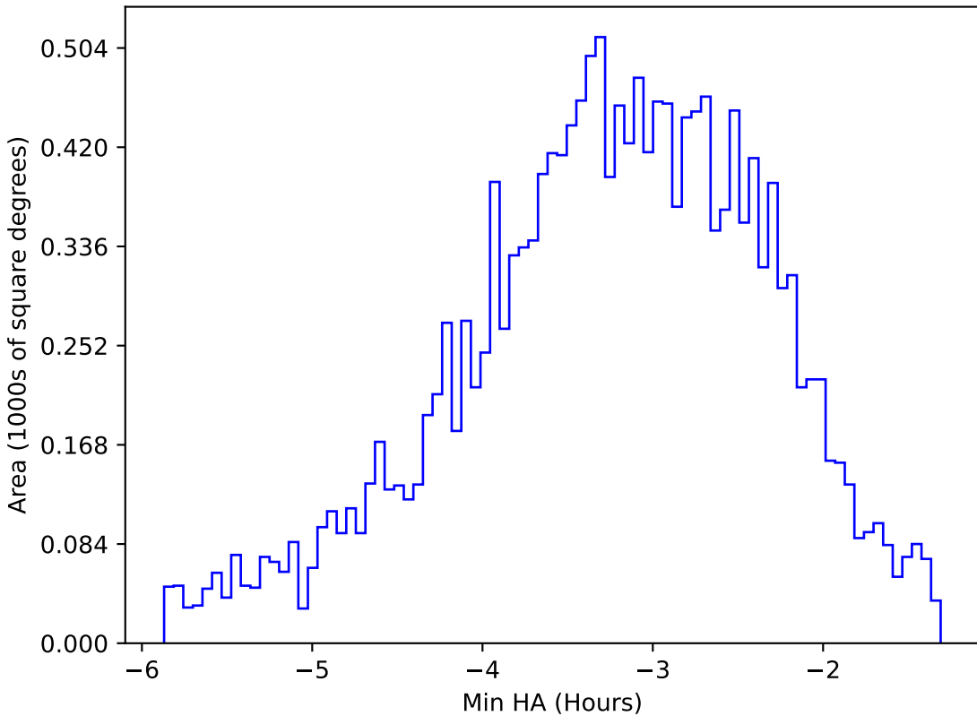
roll_pause_mjdp180_v3.4_10yrs WFD u band: Min HA
