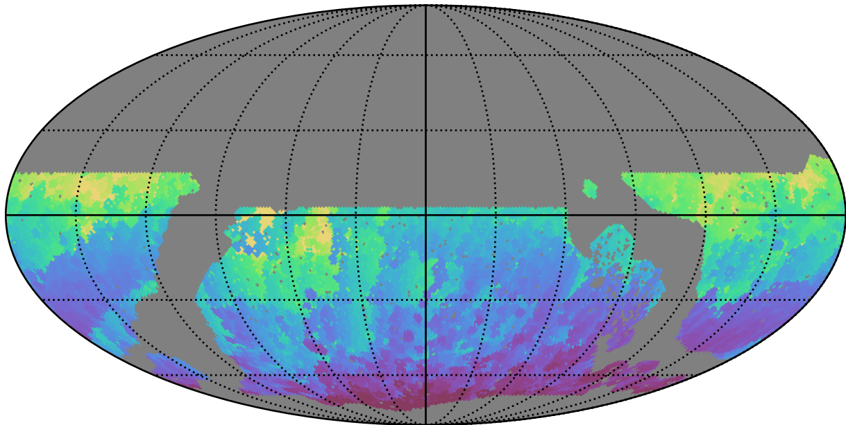
roll_pause_mjdp180_v3.4_10yrs WFD i band: Min HA
