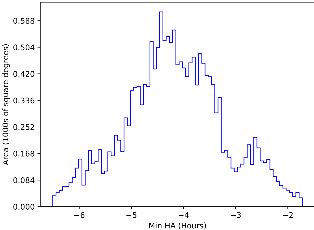
roll_pause_mjdp180_v3.4_10yrs WFD g band: Min HA
