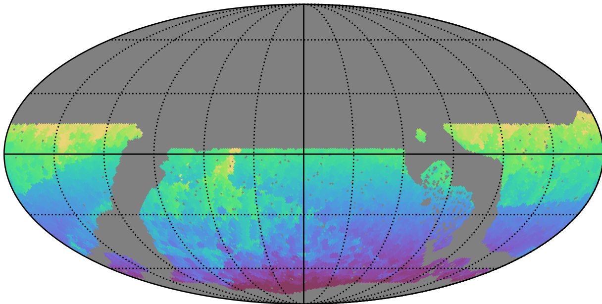
roll_pause_mjdp180_v3.4_10yrs WFD all bands: Min HA
