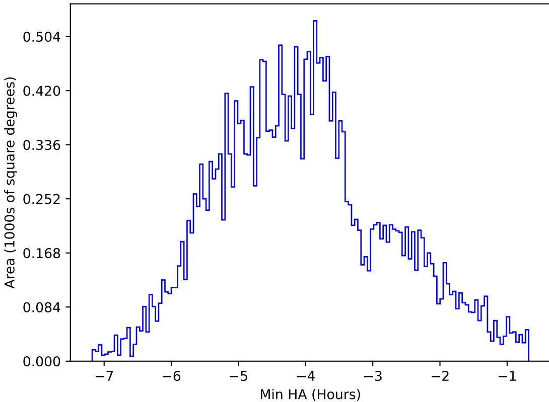
roll_pause_mjdp180_v3.4_10yrs All sky z band: Min HA
