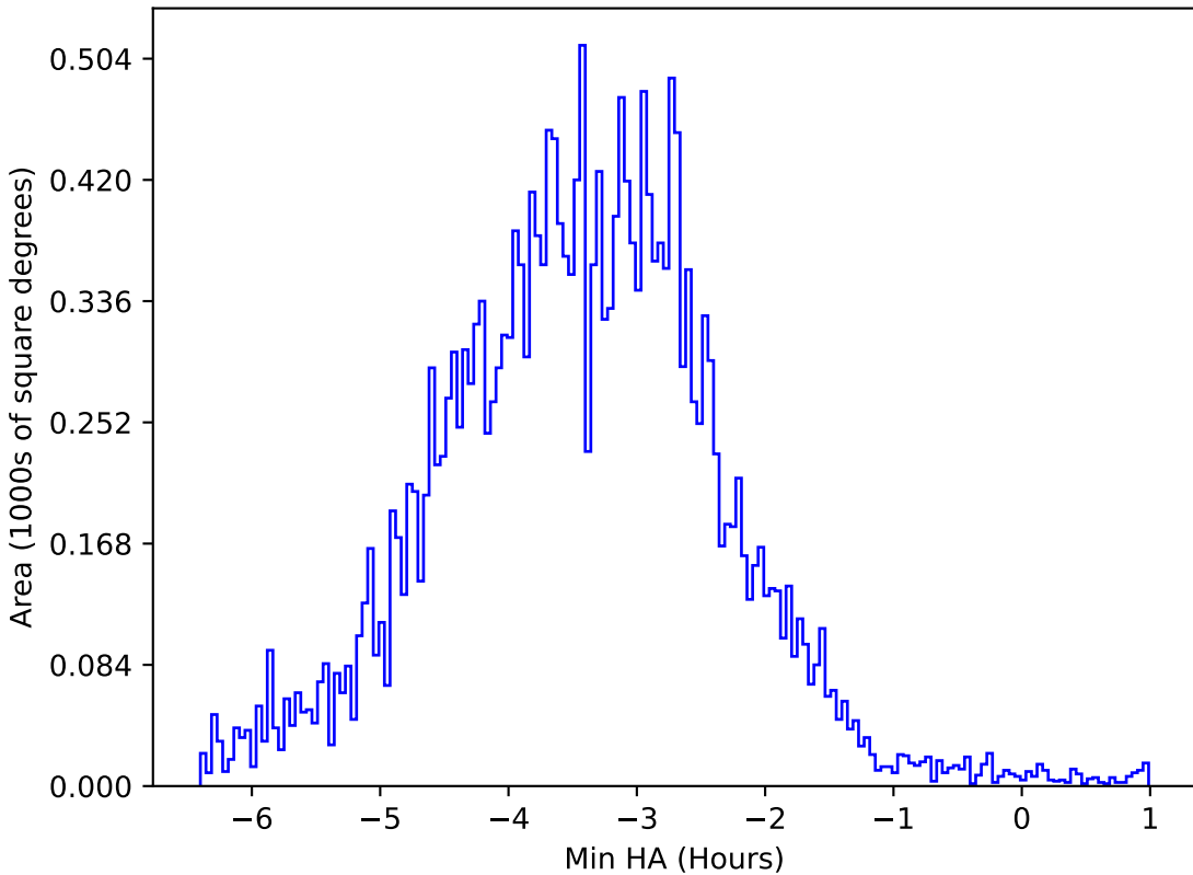
roll_pause_mjdp180_v3.4_10yrs All sky y band: Min HA
