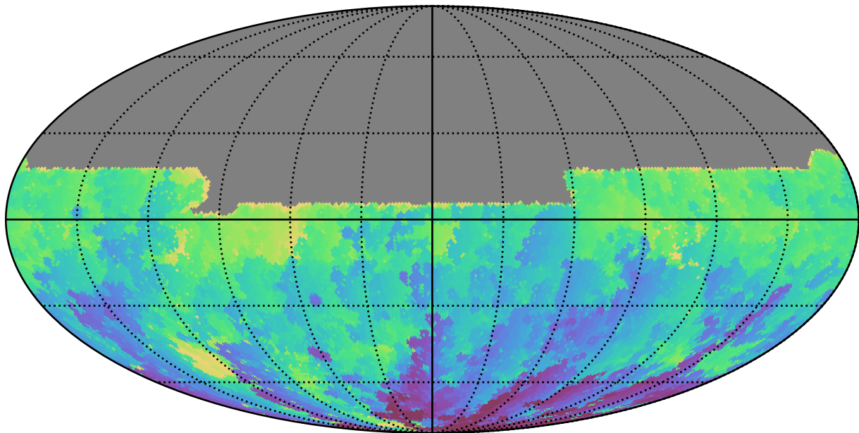
roll_pause_mjdp180_v3.4_10yrs All sky u band: Min HA
