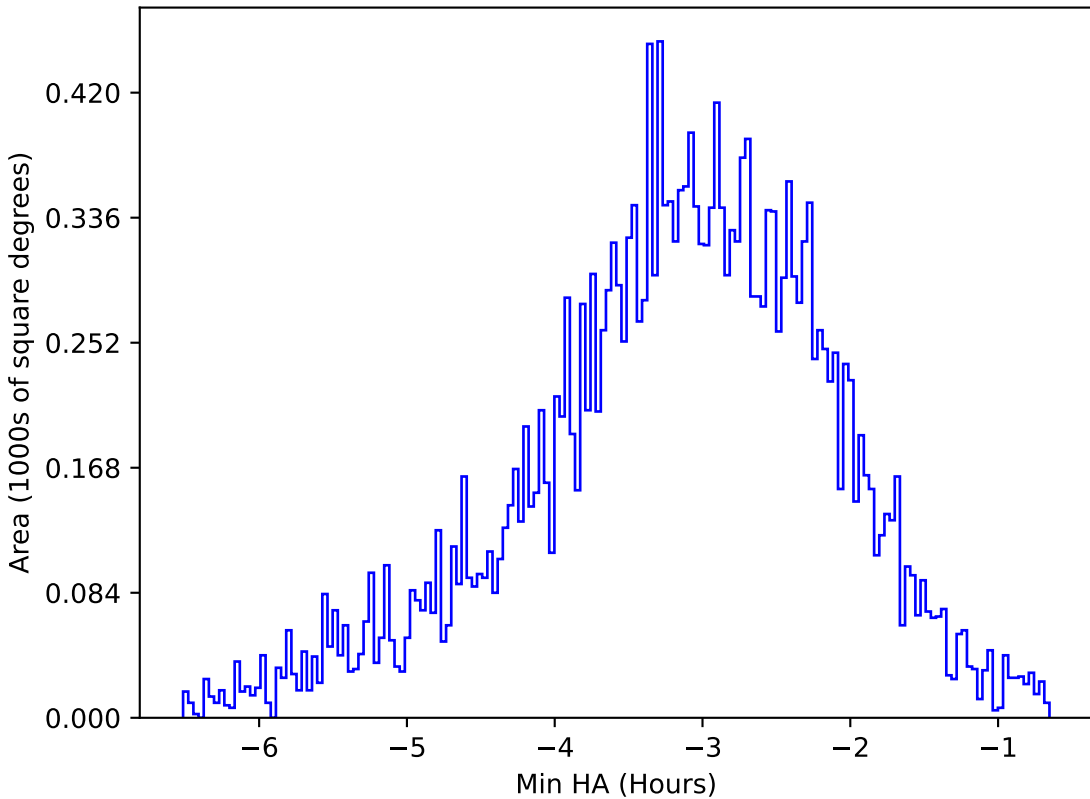
roll_pause_mjdp180_v3.4_10yrs All sky u band: Min HA
