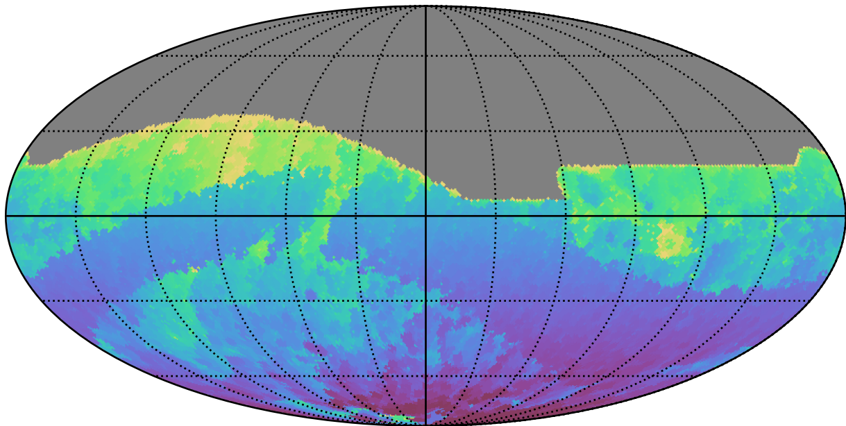
roll_pause_mjdp180_v3.4_10yrs All sky r band: Min HA
