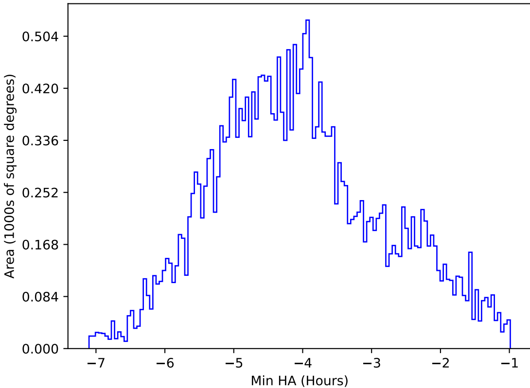
roll_pause_mjdp180_v3.4_10yrs All sky i band: Min HA
