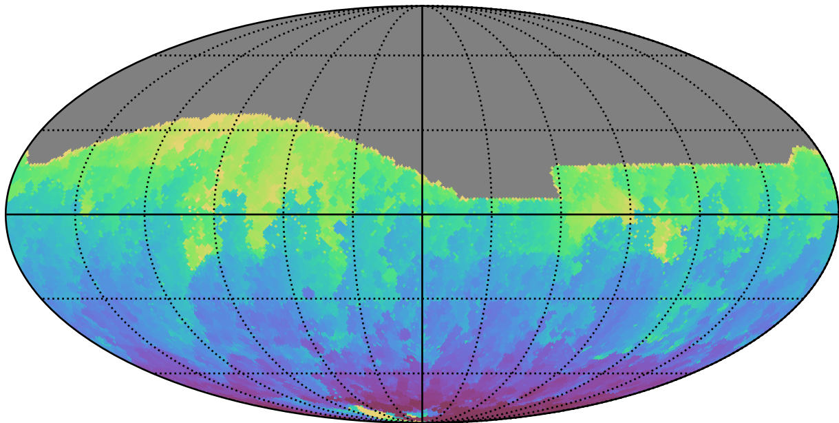
roll_pause_mjdp180_v3.4_10yrs All sky g band: Min HA
