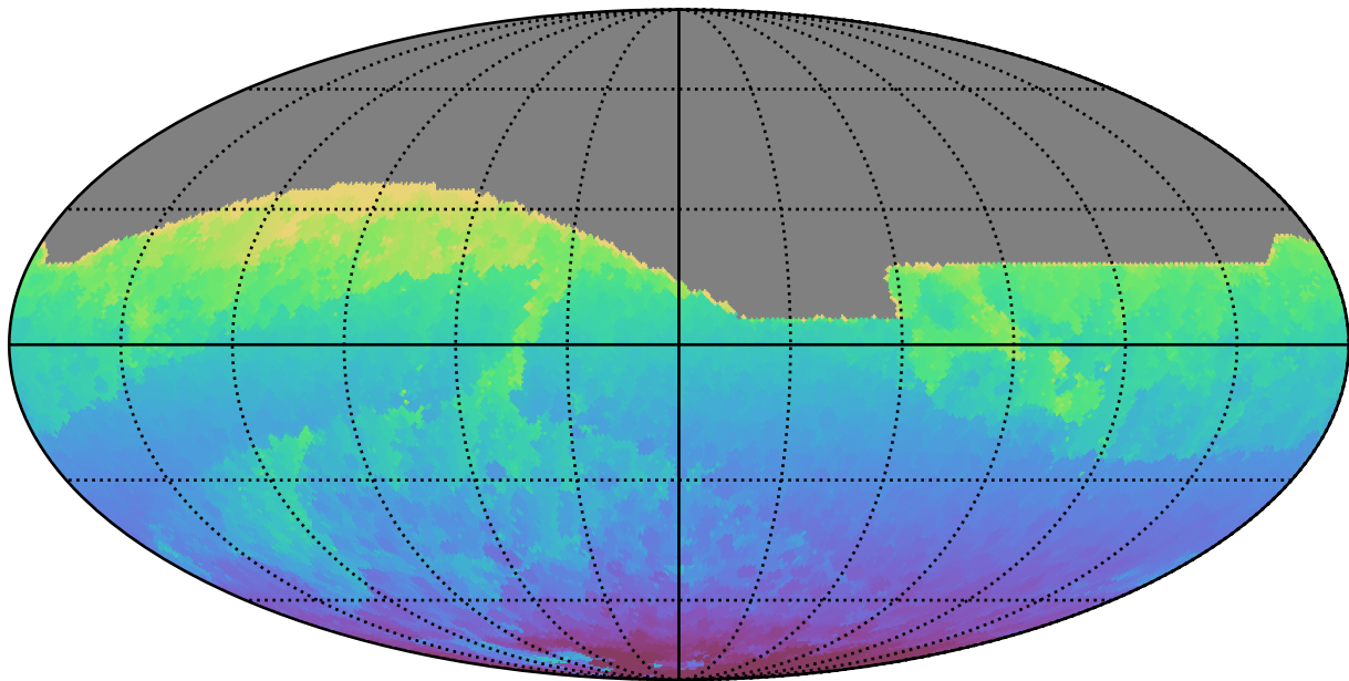
roll_pause_mjdp180_v3.4_10yrs All sky all bands: Min HA
