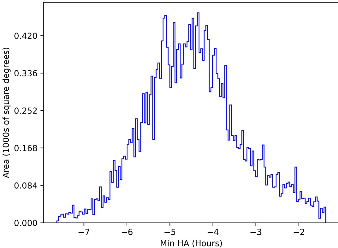
roll_pause_mjdp180_v3.4_10yrs All sky all bands: Min HA
