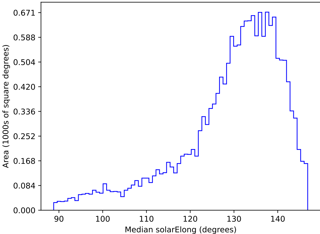
roll_pause_mjdp180_v3.4_10yrs WFD y band: Median solarElong
