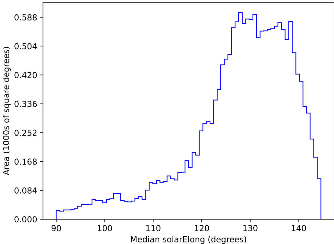
roll_pause_mjdp180_v3.4_10yrs WFD i band: Median solarElong
