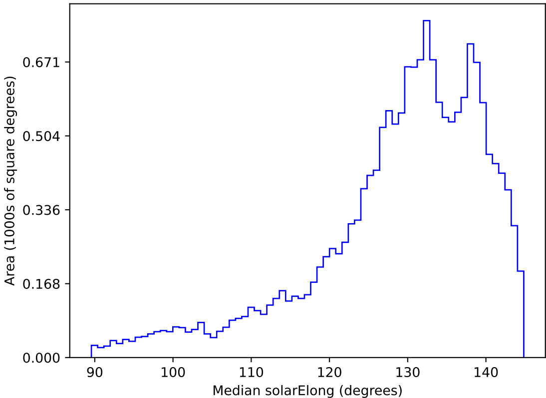
roll_pause_mjdp180_v3.4_10yrs WFD all bands: Median solarElong
