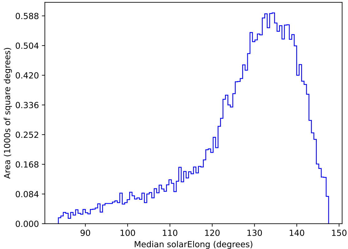
roll_pause_mjdp180_v3.4_10yrs All sky y band: Median solarElong
