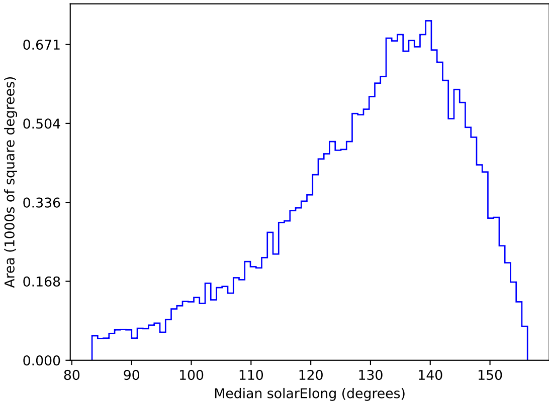
roll_pause_mjdp180_v3.4_10yrs All sky u band: Median solarElong
