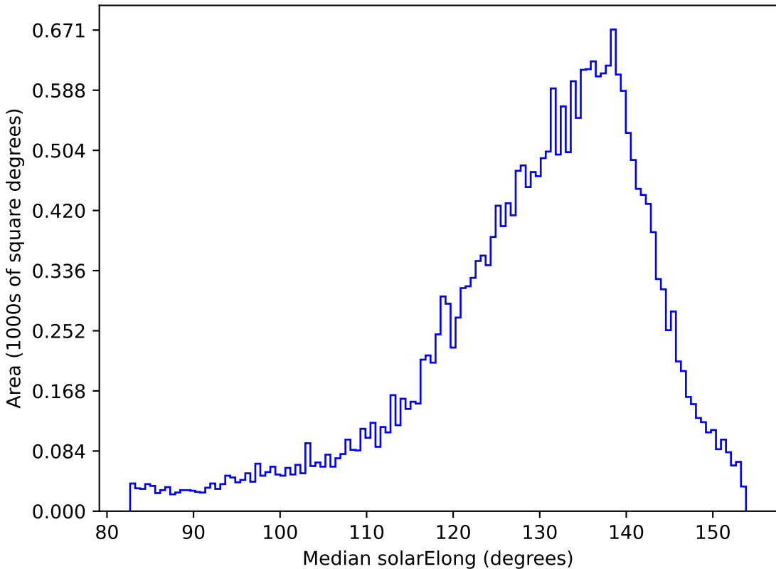
roll_pause_mjdp180_v3.4_10yrs All sky r band: Median solarElong
