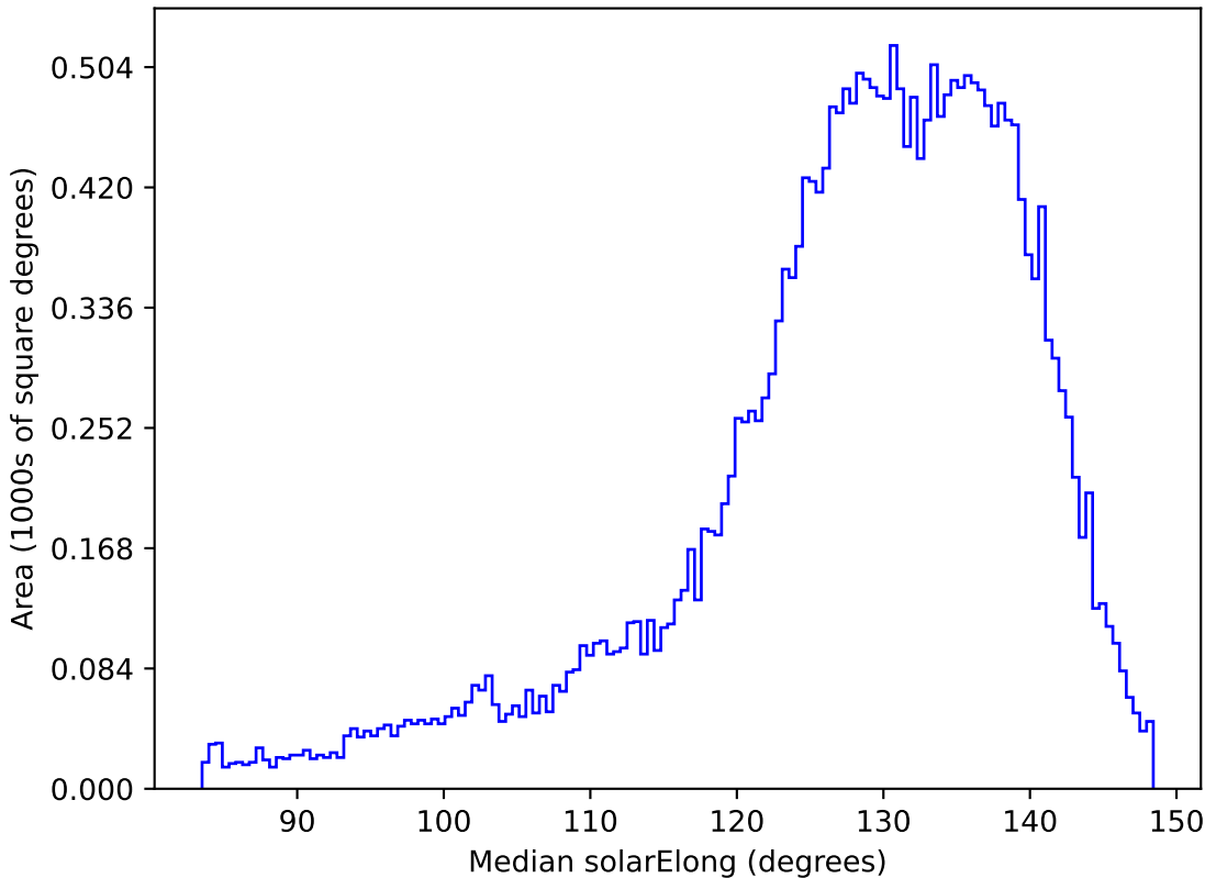
roll_pause_mjdp180_v3.4_10yrs All sky i band: Median solarElong
