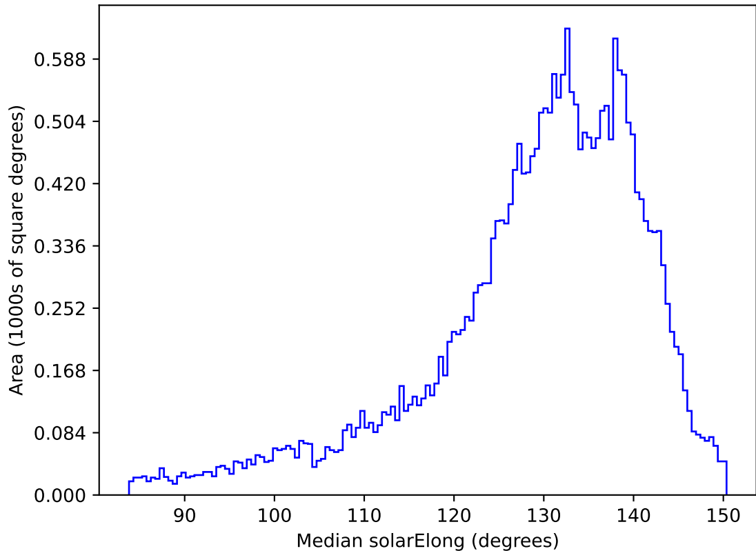
roll_pause_mjdp180_v3.4_10yrs All sky all bands: Median solarElong
