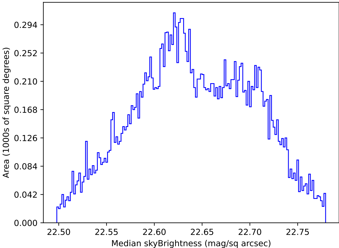
roll_pause_mjdp180_v3.4_10yrs Yr 1 u band: Median skyBrightness
