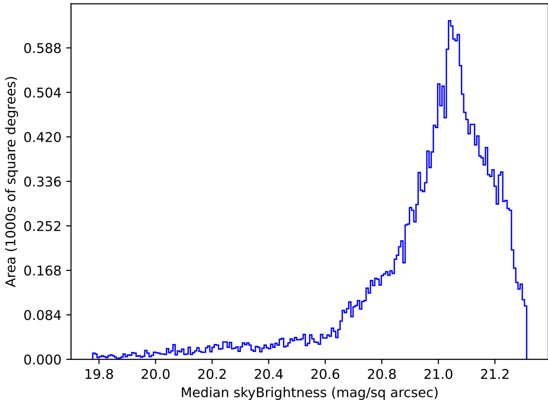
roll_pause_mjdp180_v3.4_10yrs Yr 1 r band: Median skyBrightness
