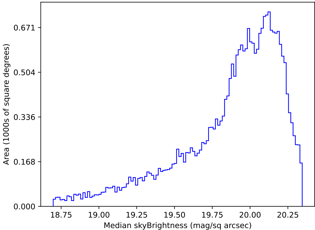
roll_pause_mjdp180_v3.4_10yrs Yr 1 i band: Median skyBrightness
