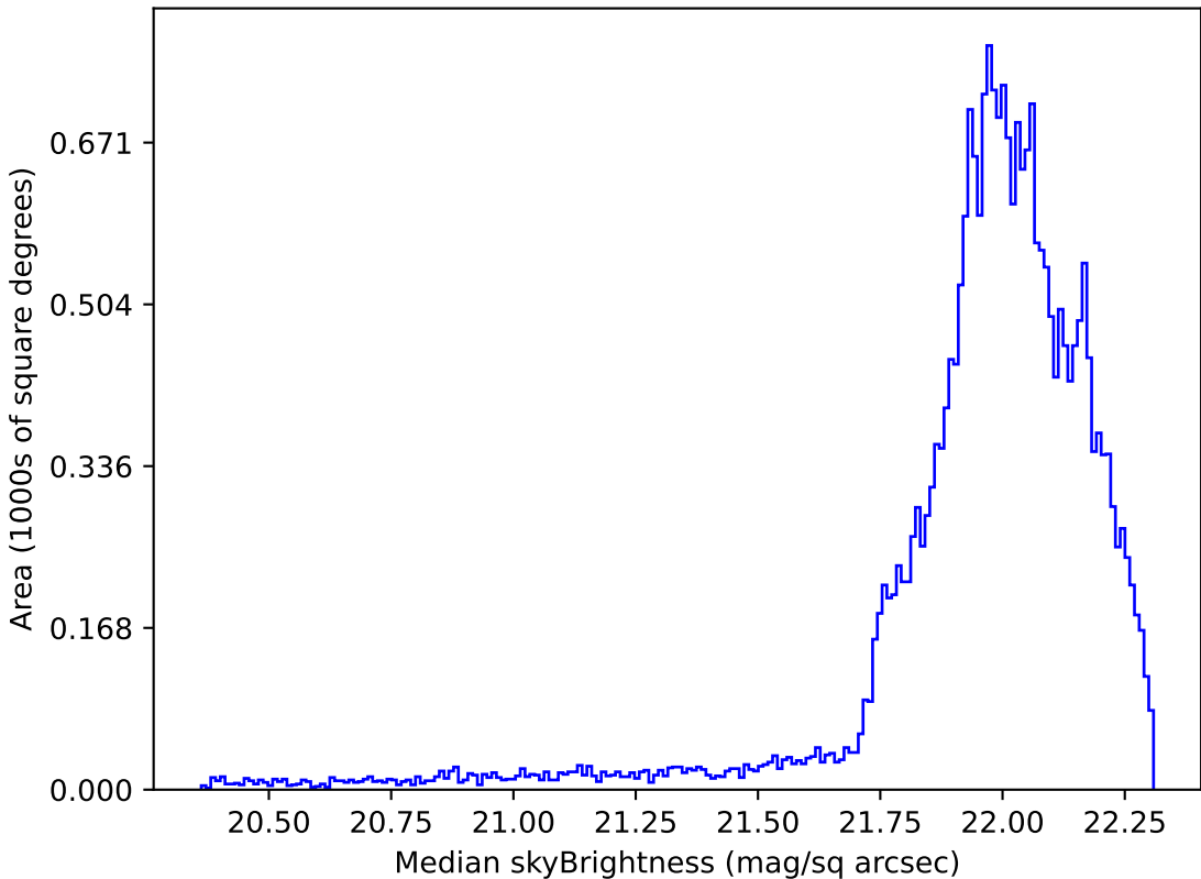
roll_pause_mjdp180_v3.4_10yrs Yr 1 g band: Median skyBrightness
