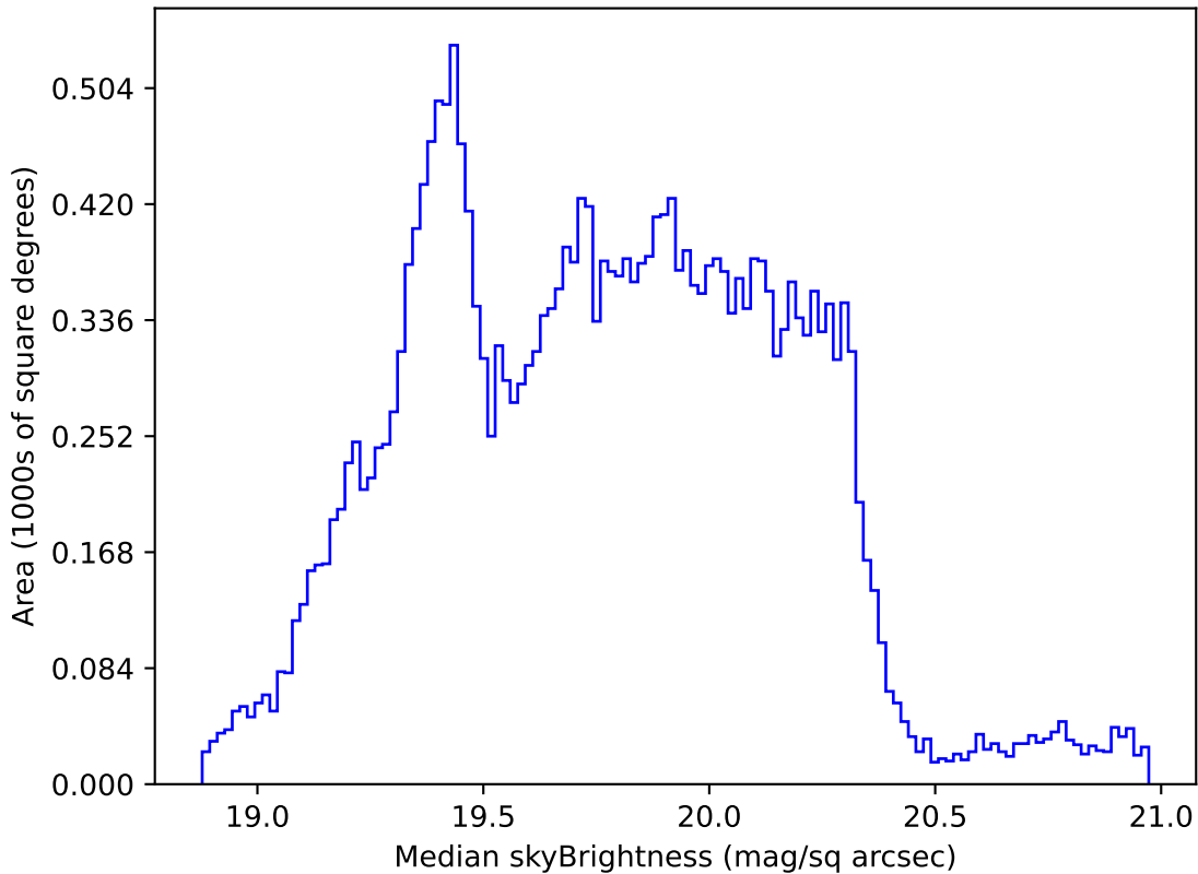
roll_pause_mjdp180_v3.4_10yrs Yr 1 all bands: Median skyBrightness
