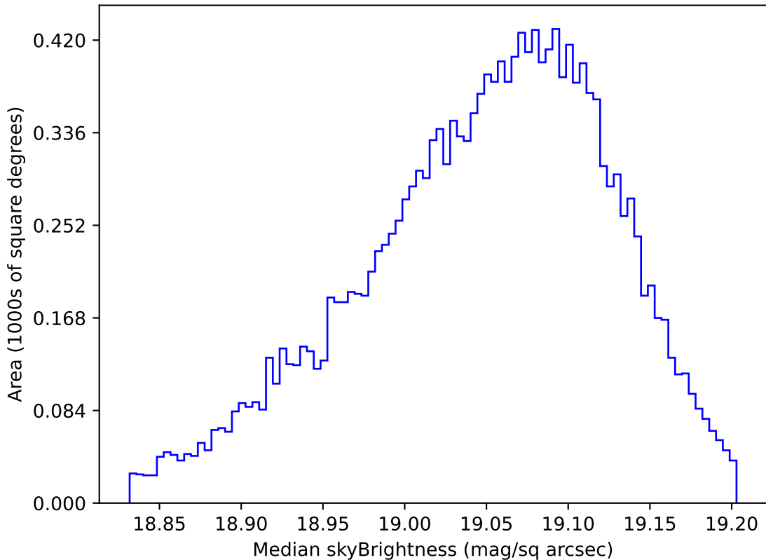
roll_pause_mjdp180_v3.4_10yrs WFD z band: Median skyBrightness
