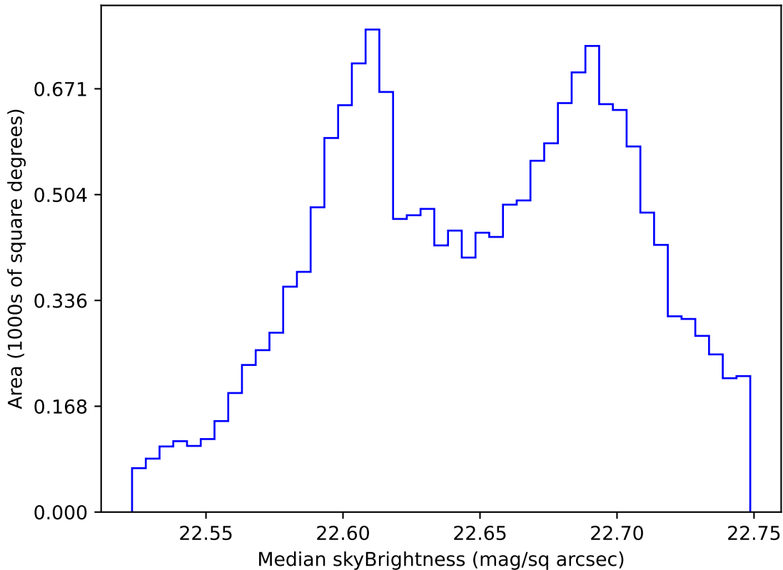
roll_pause_mjdp180_v3.4_10yrs WFD u band: Median skyBrightness
