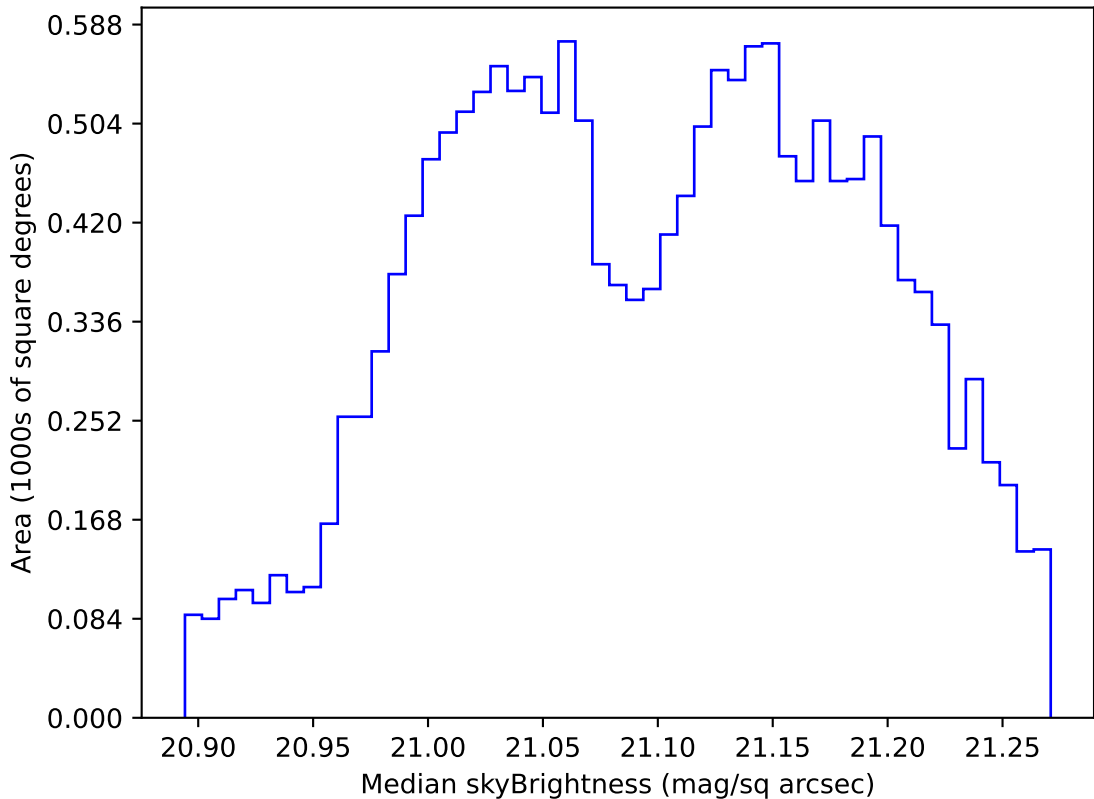
roll_pause_mjdp180_v3.4_10yrs WFD r band: Median skyBrightness
