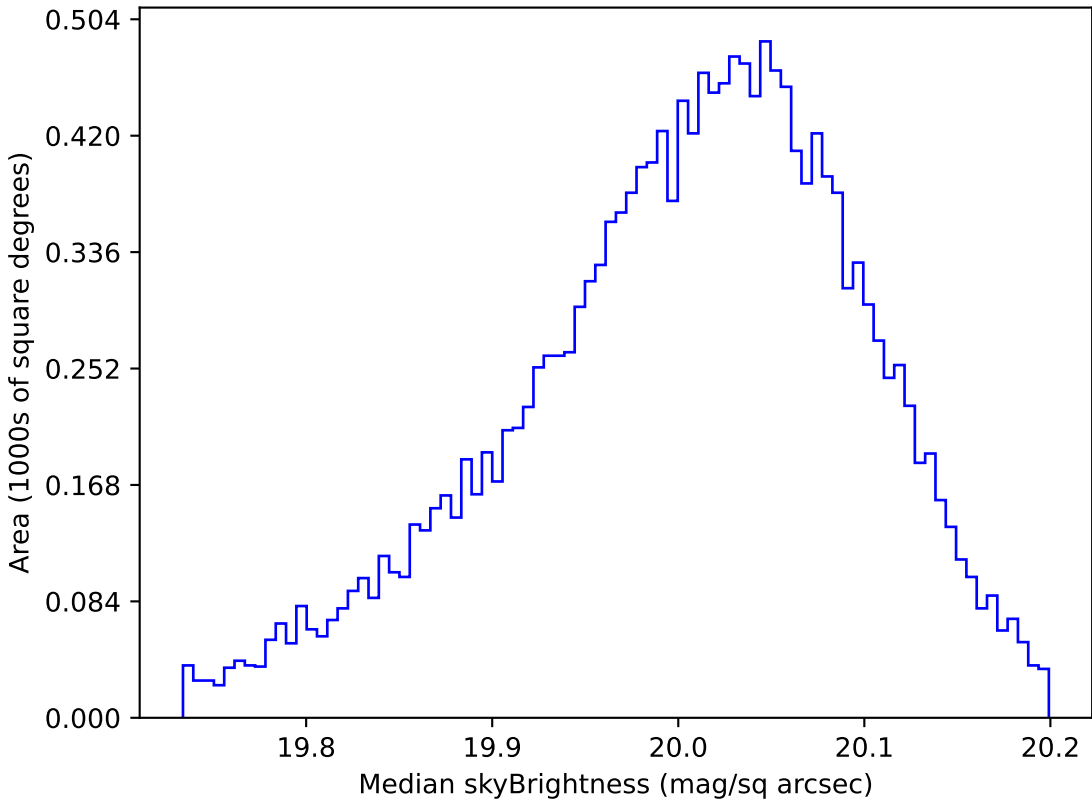
roll_pause_mjdp180_v3.4_10yrs WFD i band: Median skyBrightness
