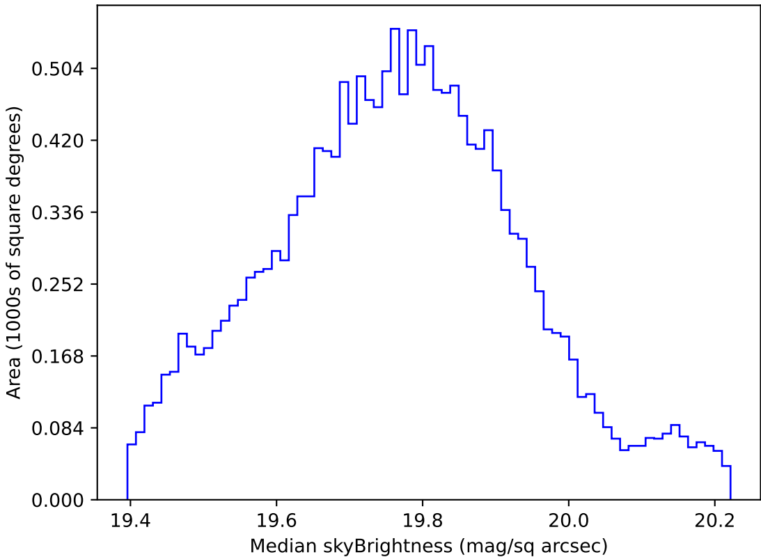
roll_pause_mjdp180_v3.4_10yrs WFD all bands: Median skyBrightness
