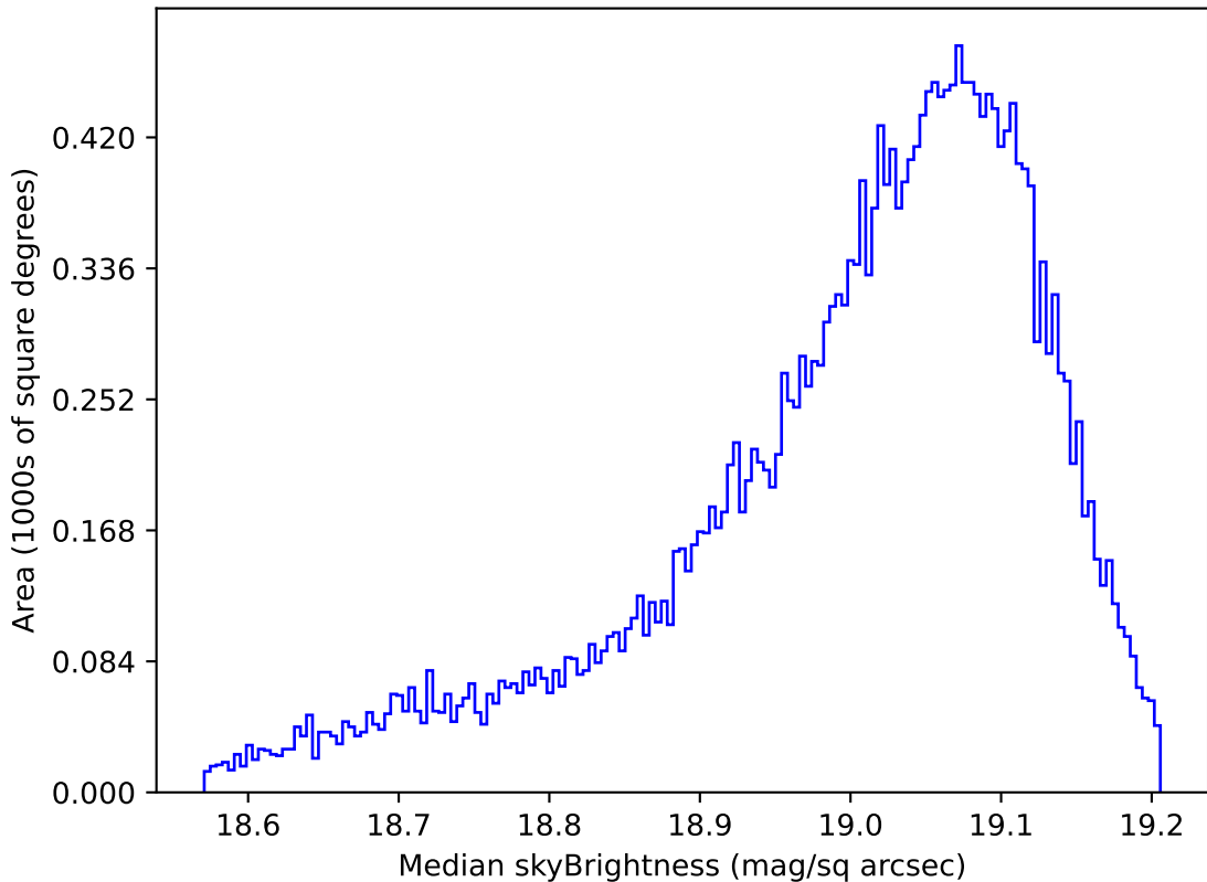
roll_pause_mjdp180_v3.4_10yrs All sky z band: Median skyBrightness
