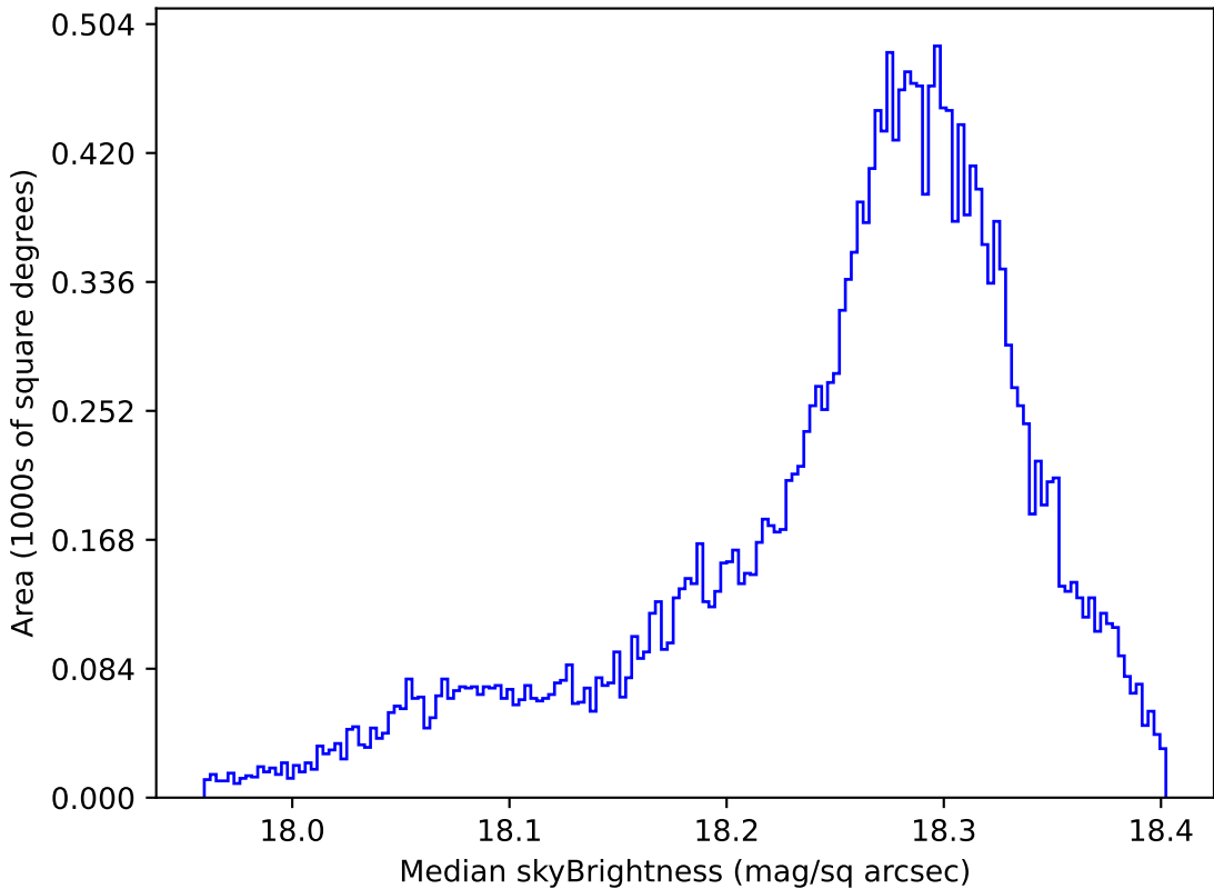
roll_pause_mjdp180_v3.4_10yrs All sky y band: Median skyBrightness
